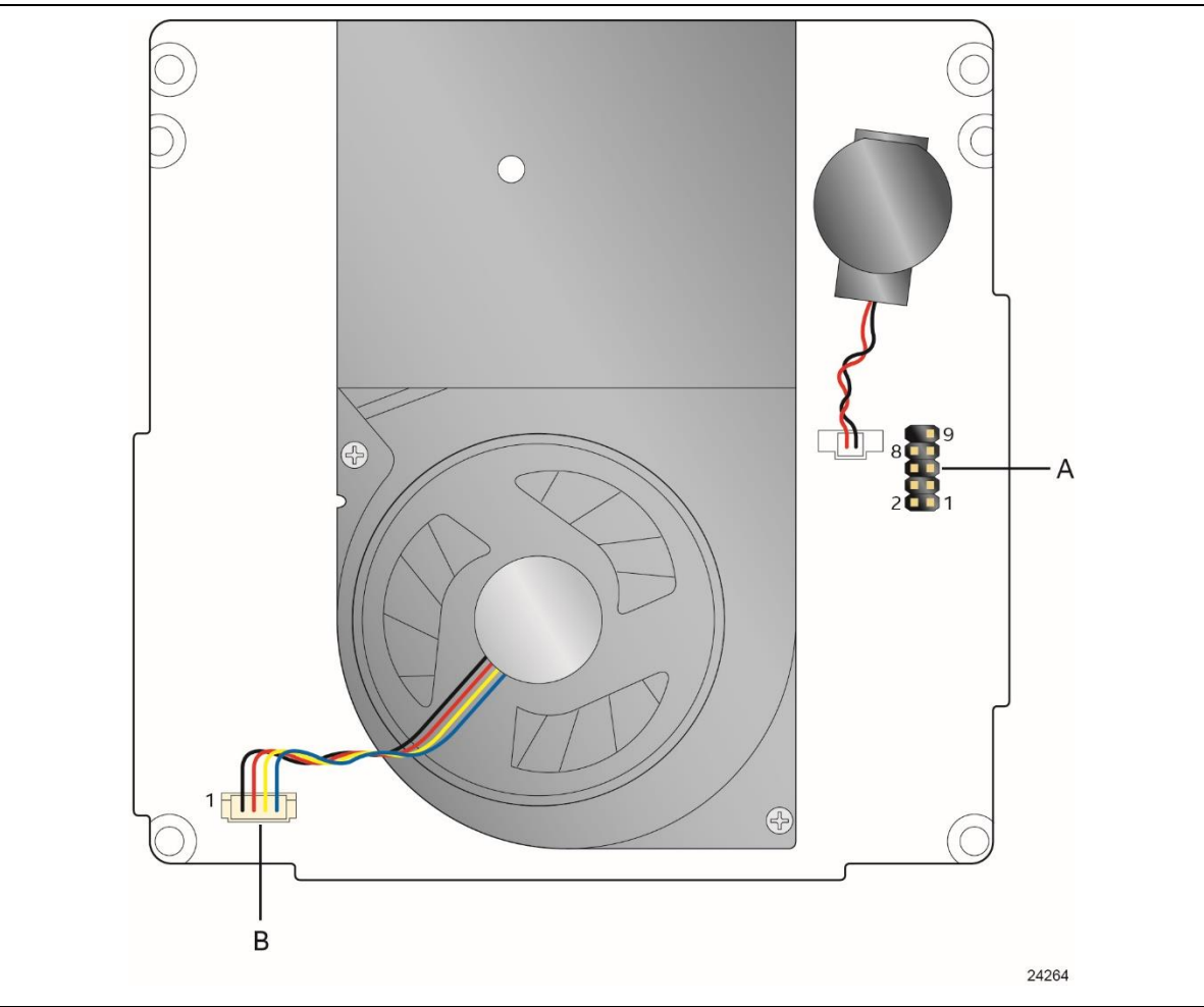
Figure 12. Headers and Connectors (Top)
